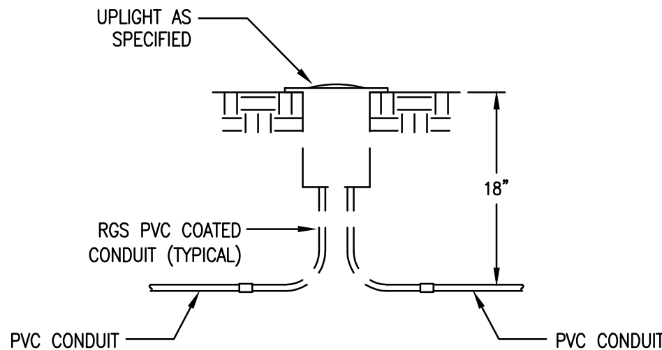
UPLIGHT MOUNTING DETAIL Scale: NTS
