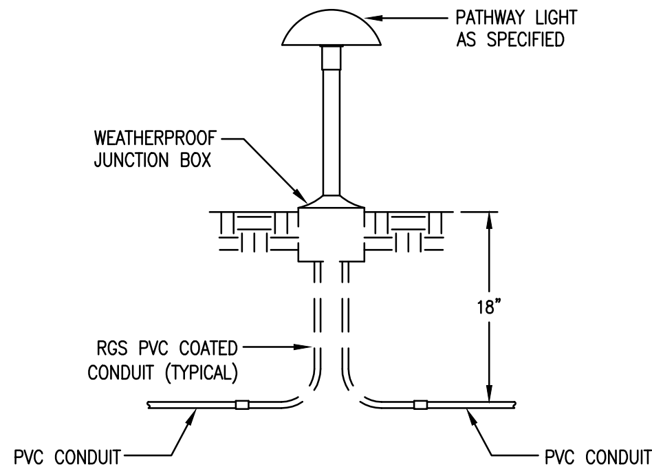
PATHWAY LIGHT MOUNTING DETAIL Scale: NTS
