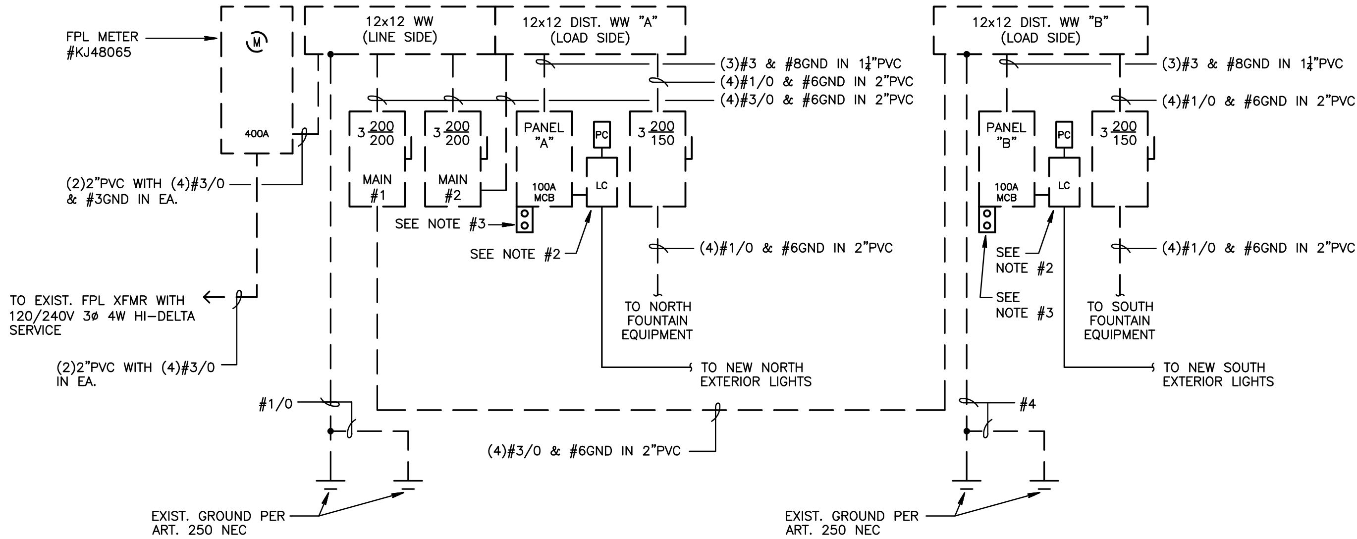
ELECTRICAL RISER DIAGRAM Scale: NTS
