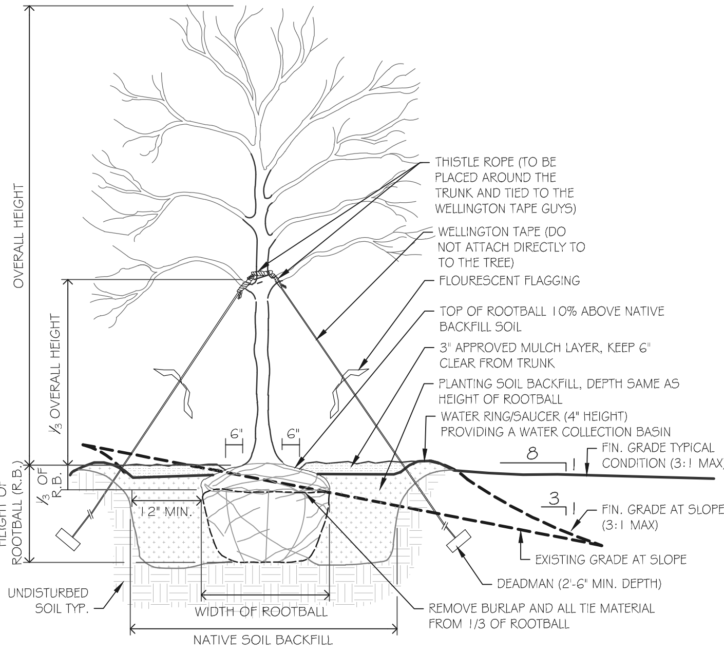
1 TREE PLANTING DETAIL
