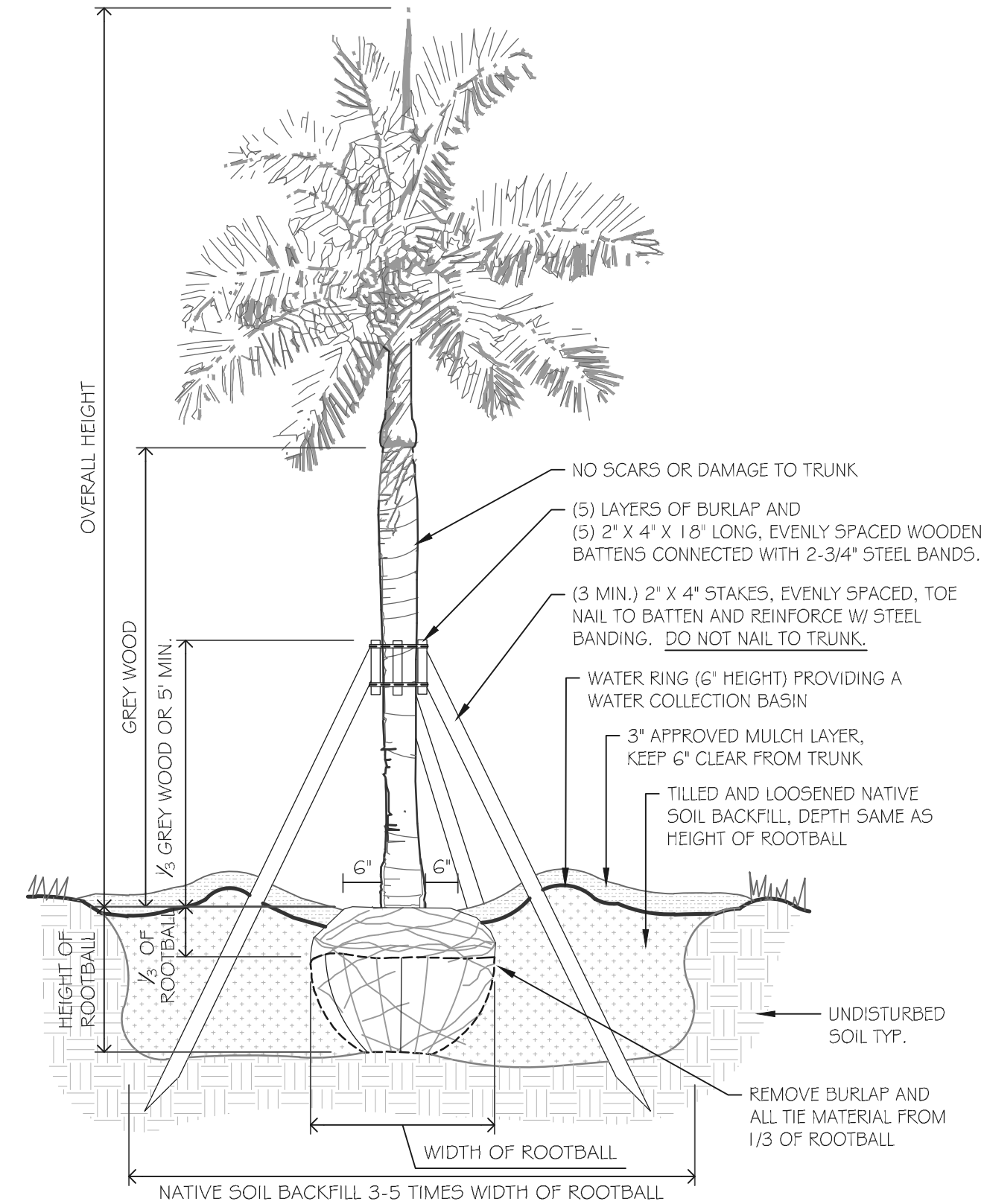
2 PALM PLANTING DETAIL
