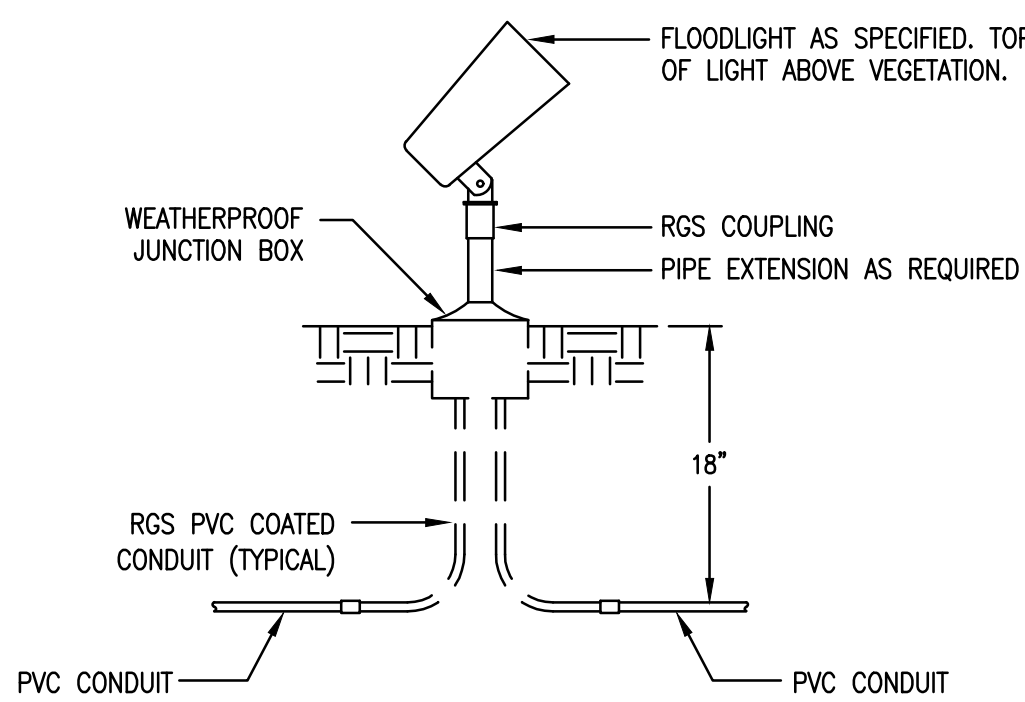
FLOODLIGHT MOUNTING DETAIL Scale: NTS
