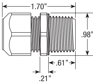
Cord Grip
