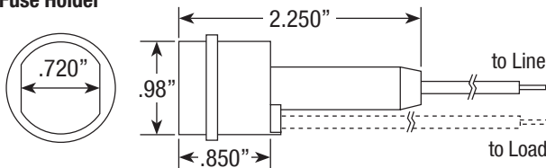
Fuse Holder
